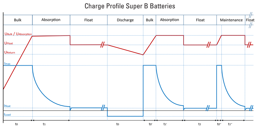
Figure 18. Charge curve
