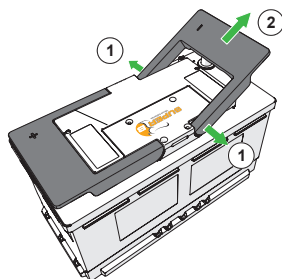
Figure 11. Remove the handles by pulling them outwards.
