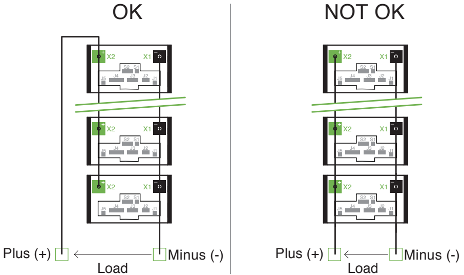
Figure 17. Connecting batteries in parallel
