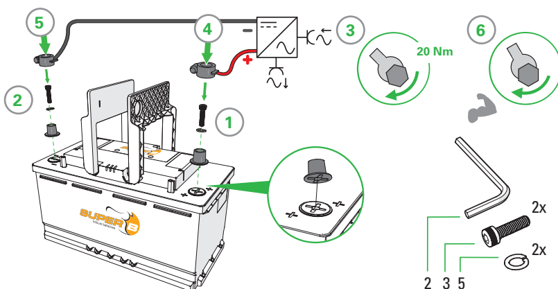
Figure 5. Connecting power cables with automotive type terminals
