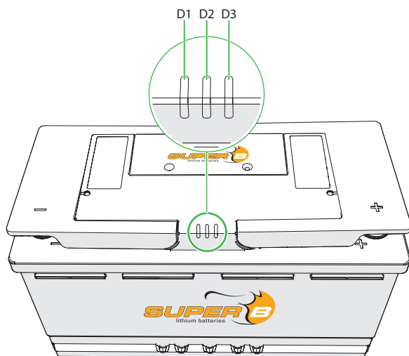
Figure 4. LED Indicators
