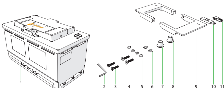
Figure 2. Components
