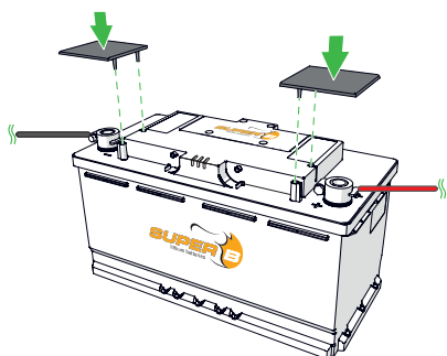
Figure 13. Place the accessory caps over that terminals. Accessory caps are not provided by Super B
