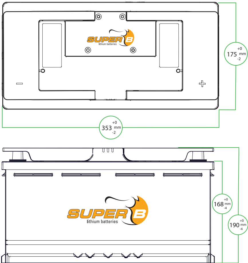
Figure 1. Dimensions
